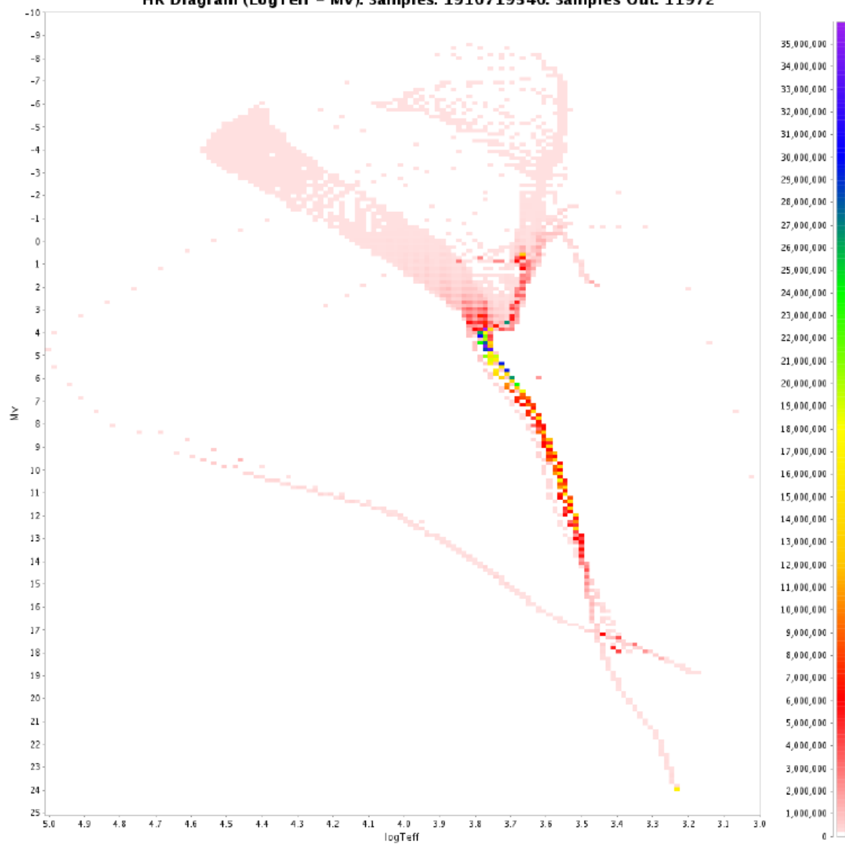
HR Diagram (LogTeff - Mv). Samples: 1910719540. Samples Out: 11972
